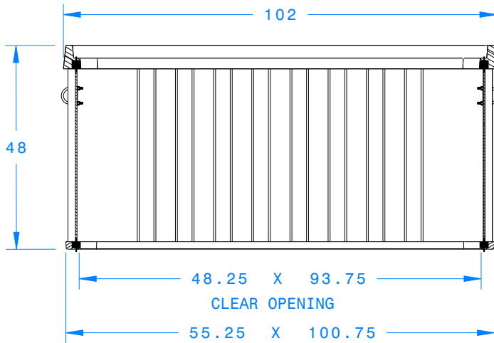
ASSEMBLY SECTION
